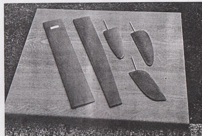
1MTR CARBON FIBRE FINS AND RUDDERS
